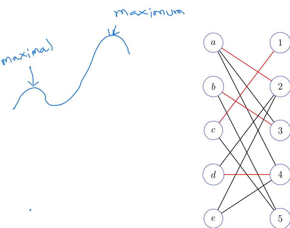
Figure 2: The red edges form a maximal matching for the bipartite graph.
