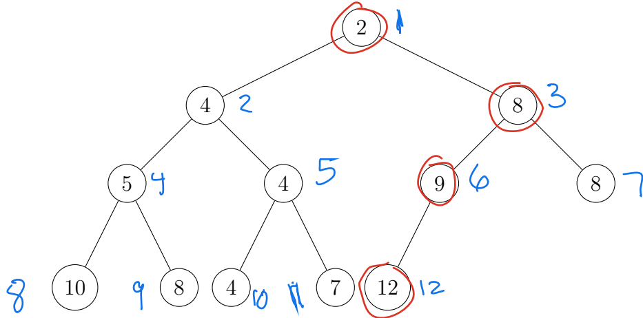
Example of a binary min heap whose nodes store integers.
