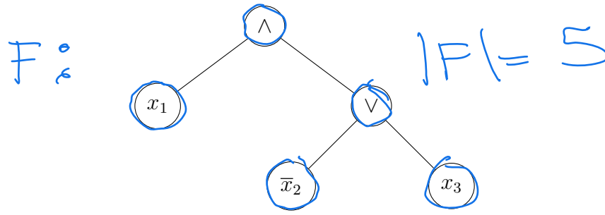
Figure 2: Parse tree for Boolean formula x_1 \wedge (\bar{x}_2 \vee x_3)
